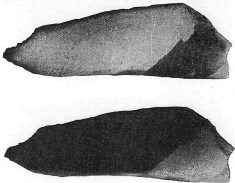
FIG. 5. Photographs taken at different angles of the smaller polished and etched surface ( 3 \times 1 cm.) of the Hoba meteoric iron, showing the oriented sheen. Photographs by H. G. Herring. \times 3 .
